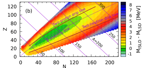
Fig. 2: Difference of the atomic mass estimates obtained using the LSD [38] the ISLD(b) the LSD [38] models.
