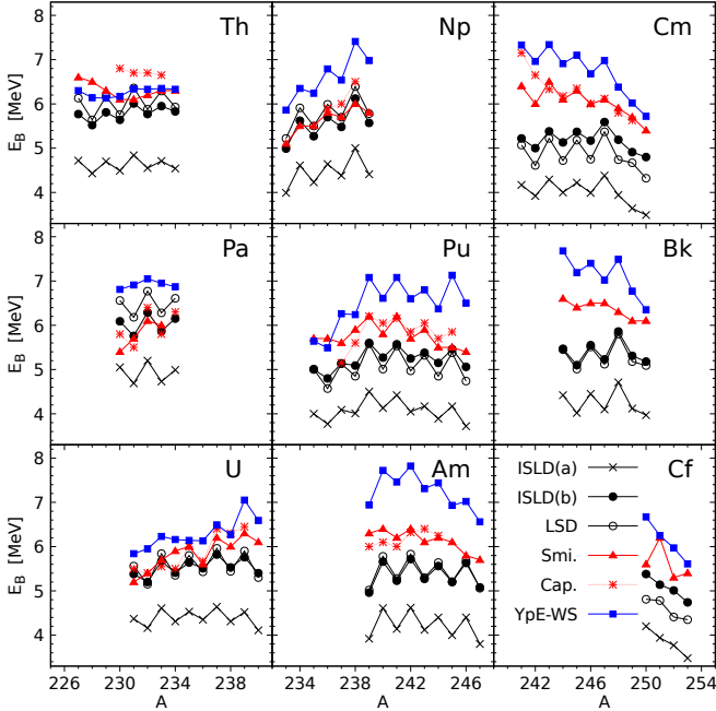
Fig. 4: Fission barrier heights evaluated using the topographical theorem [39] with the ISLD(a) (crosses), ISLD(b) (points), and LSD (open circles) set of parameters are compared with the empirical/experimental data taken from Ref. [58] (triangles) and [59] (stars) and with the theoretical values obtained within the mac-mic model in Ref. [60].
