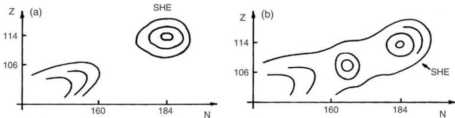
Fig. 8. Regions of relatively long-lived heavy nuclei as believed earlier (a), and after inclusion of higher multipolarity deformations (b). The figure taken from Ref. [11].
