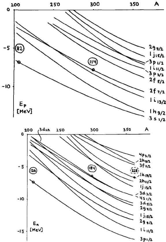
Fig. 2. Proton (top) and neutron (bottom) single-particle energies obtained with the Woods-Saxon potential as a function of the mass number A . The plots taken from Ref. [1].
