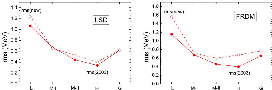
Fig. 16. R.m.s. deviation of LSD (l.h.s.) and FRDM (r.h.s.) estimates from the experimental data available in 2003 (solid line) and in 2017 (dashed line). The symbols: L, M-I, M-II, H and G denote the regions of light, medium-I, medium-II, heavy, and all considered nuclei, respectively (figures taken from Ref. [25]).
