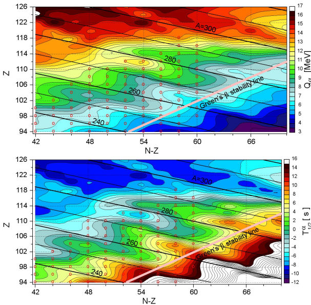
Fig. 8. Q_\alpha values (top) and \alpha -decay half-lives T_{1/2}^\alpha (bottom) for the region of super-heavy elements.
