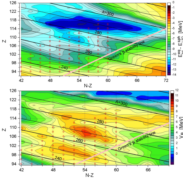
Fig. 7. Microscopic energy corrections in the ground states of the nuclei in the super-heavy region (top) and fission barrier heights (bottom).
