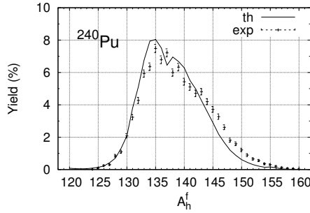
Fig. 4. Comparison between the fission-fragment mass yield of ^{240}\text{Pu} obtained in our approach with the experimental data [10].
