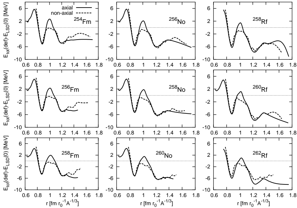
Fig. 1. The total deformation energy defined by the difference E_{\text{tot}} - E_{\text{LSD}}(0) , along the fission path found by minimisation of the total energy with respect to \{\alpha_{2,0}, \alpha_{2,2}, \alpha_{4,0}, \alpha_{4,2}, \alpha_{4,4}\} - non-axial case (dashed lines) and \{\alpha_{2,0}, \alpha_{4,0}, \alpha_{6,0}, \alpha_{8,0}, \alpha_{10,0}\} axial case (solid lines) for Fm, No and Rf isotopes.
