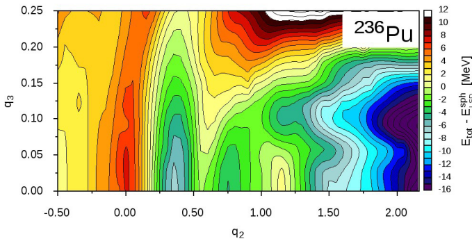
Fig. 1. Potential energy surface of ^{236}\text{Pu} on the (q_2, q_3) plane.
