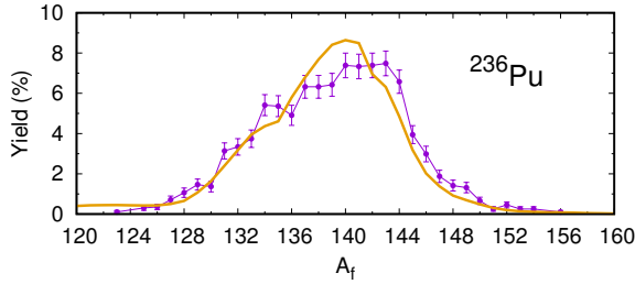
Fig. 3. Experimental fission fragment mass yield for the spontaneous fission of ^{236}\text{Pu} [8] compared with our estimate (2.6) for E_0 = 2 MeV.
