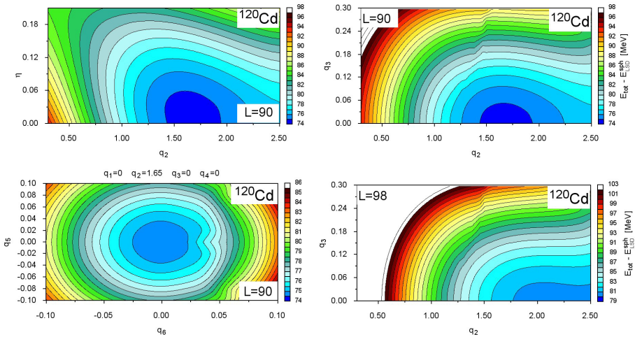
Fig. 4. The same as in Fig. 3 but for higher angular momenta.
