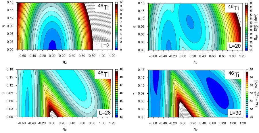
Fig. 1. Potential energy landscape of ^{46}\text{Ti} in the (q_2, \eta) plane for the low angular momenta L = 2, 20, 28 , and 30 \hbar .
