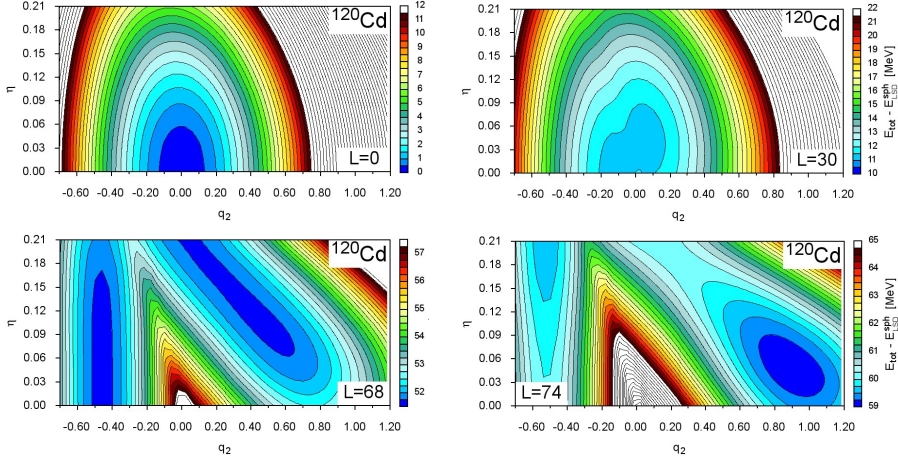
Fig. 3. Potential energy landscape of ^{120}\text{Cd} in the (q_2, \eta) plane for the low angular momenta L = 0, 30, 68 , and 74 \hbar .
