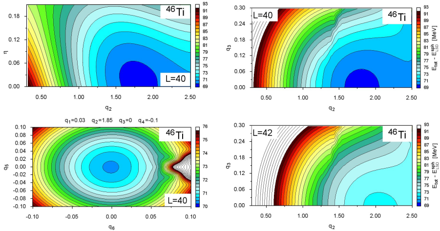
Fig. 2. The same as in Fig. 1 but for higher angular momenta.
