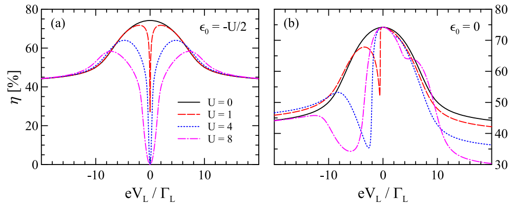
Fig. 2 Dependence of the CPS efficiency \eta on the voltage V_L for \Gamma_S/\Gamma_L = 16 , \Gamma_R/\Gamma_L = 4 , V_R = 0 , T = 0 , U/\Gamma_L = \{0, 1, 4, 8\} and a \epsilon_0 = -U/2 and b \epsilon_0 = 0
