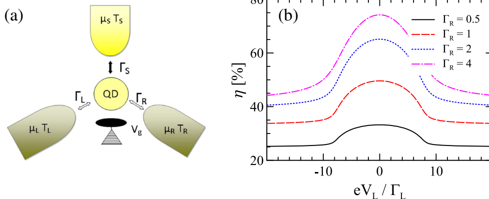
Fig. 1 a Sketch of the system. b Efficiency \eta with respect to V_L for \Gamma_S/\Gamma_L = 16 , \epsilon_0 = 0 , U = 0 , V_R = 0 , T = 0 and \Gamma_R/\Gamma_L = \{0.5, 1, 2, 4\} . \Gamma_L is treated as unity in our calculations
