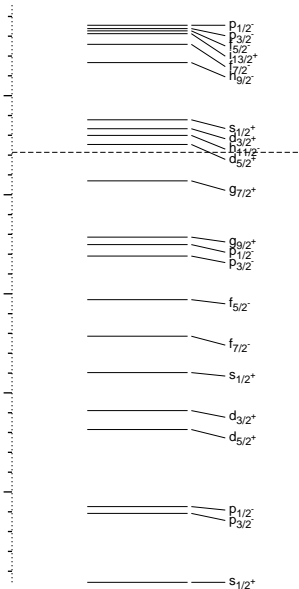
^{144}\text{Nd}_{84}, p
