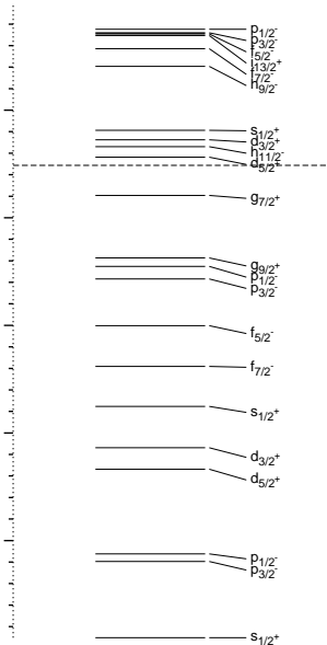
^{142}\text{Nd}_{82}, p
