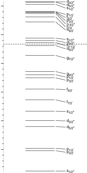
^{150}_{66}\text{Dy}_{84}, p
