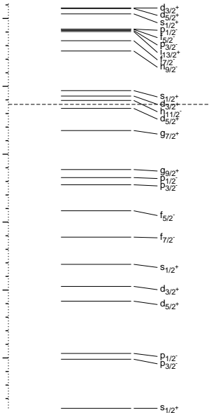
^{148}_{66}\text{Dy}_{82}, p
