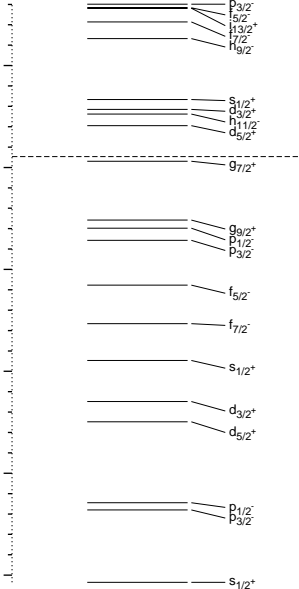
^{140}_{56}\text{Ba}_{84}, p
