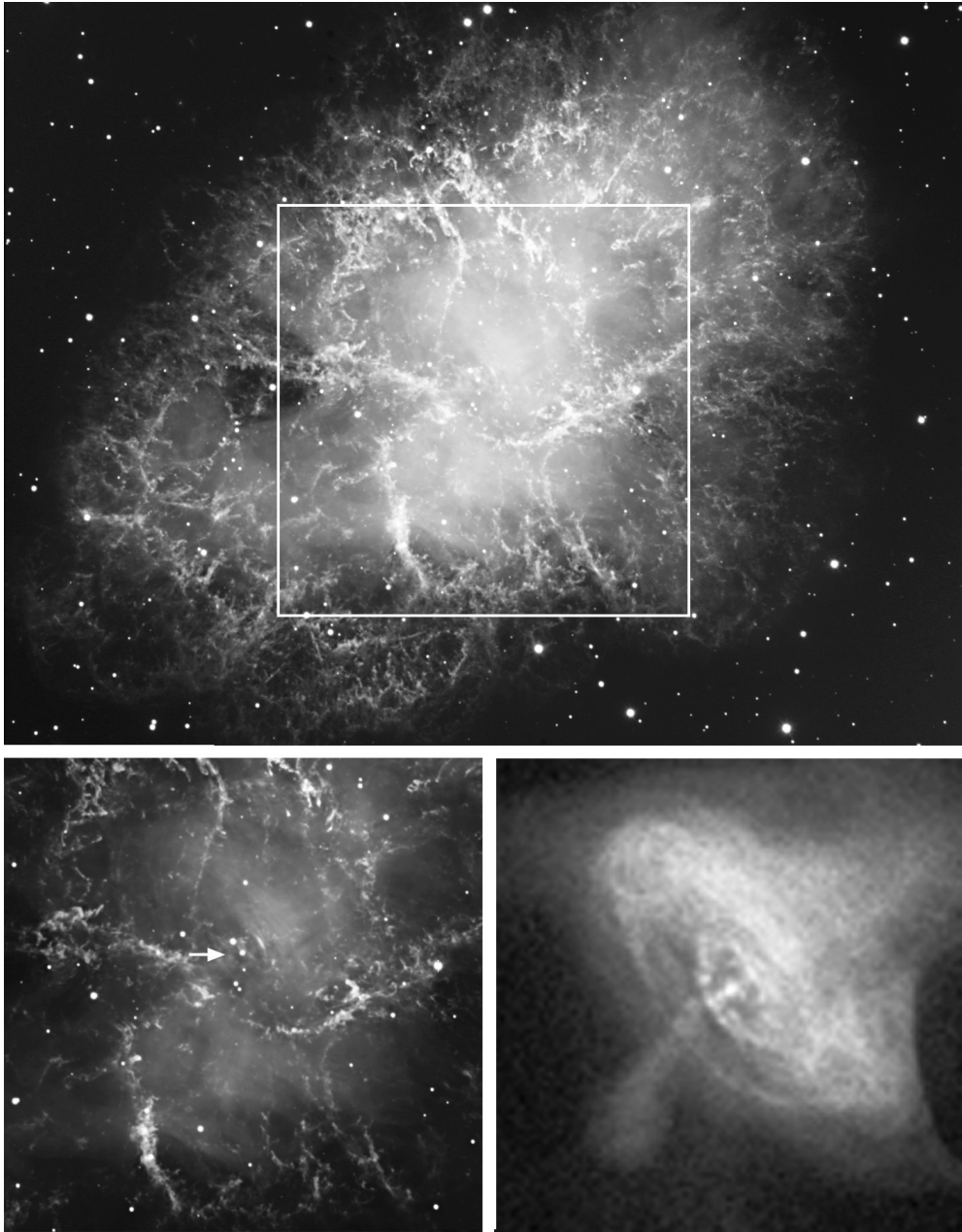
Figure 4.11 The Crab nebula, the remnant of a core-collapse supernova that exploded in the year 1054, at a distance of 2 kpc. Top: Image in optical light. Image scale is 4 pc on a side. Bottom: Zoom-in on the area marked in the top photo, in optical light ( left ), with the pulsar at the center of the remnant indicated by the arrow; and in X-rays ( right ), showing the pulsar, bidirectional jets, and a toroidal structure formed by synchrotron emission from energetic particles. Note that a similar emission morphology is faintly discernible also in the optical image on the left. Photo credits: European Southern Observatory; and NASA/CXC/ASU and J. Hester et al.
