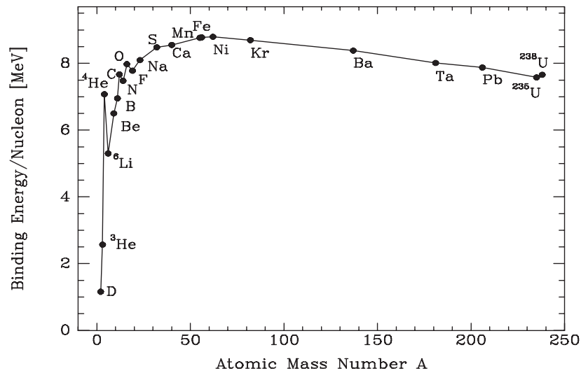
Figure 4.8 Binding energy per nucleon as a function of atomic mass number. Several elements are marked. The iron-group elements with A \approx 56 have the highest binding energy per nucleon, 8.8 MeV, and therefore nuclear fusion of these elements into heavier elements does not release thermal energy, but rather consumes it.
