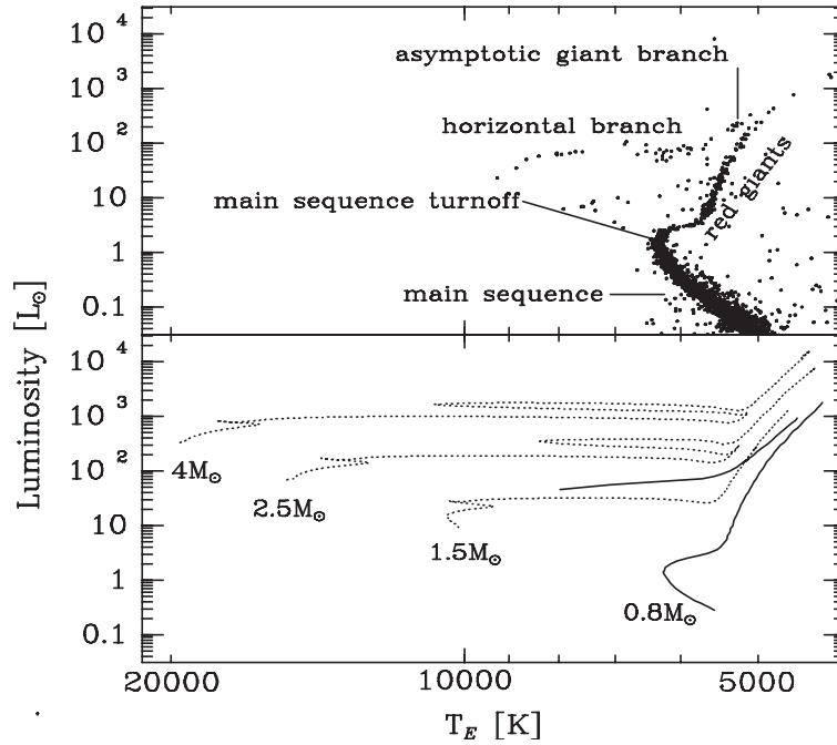
Figure 4.1 Illustration of post-main-sequence evolution on the H-R diagram. Top: Observed H-R diagram for stars in the globular cluster M3 (more on star clusters in chapter 5.1.4). The main-sequence turnoff marks the point at which stars are now leaving the main sequence and evolving onto the red-giant branch. All the stars in the cluster formed together about 13 Gyr ago, and the cluster has not experienced subsequent star formation. As a result, all stars above a certain mass, corresponding to the turnoff point, have left the main sequence, while those below that mass are still on the main sequence. The density of points in each region of the diagram reflects the amount of time spent by stars in each post-main-sequence evolution stage. Bottom: Theoretical stellar evolution tracks for stars of various initial main-sequence masses (with an assumed initial metal abundance of Z = 0.0004 ). Each track begins at the lower left end on the zero-age main sequence . After leaving the main sequence, stars evolve along, and up to the tip of, the red-giant branch. They then move quickly on the diagram to the left edge of the horizontal branch , where helium core burning and hydrogen shell burning take place, and evolve to the right along the horizontal branch. Once all the helium in the core has been converted to carbon and oxygen, the star rises up the “asymptotic giant branch” where double shell burning—a helium-burning shell within a hydrogen-burning shell—takes place. Note the good correspondence between the theoretical track for the 0.8M_{\odot} initial-mass star (solid line) and the observed H-R diagram on top. For clarity, the theoretical horizontal and asymptotic giant branches are not shown for the other initial masses. Data credits: S.-C. Rey et al. 2001, Astrophys. J. , 122, 3219; and L. Girardi, et al. 2000, Astron. Astrophys. Suppl. , 141, 371.
