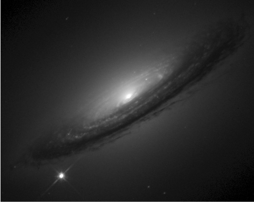
Figure 4.9 Optical-light image of the supernova SN1994D, below and to the left of its host galaxy, NGC 4526. For several weeks around its peak brightness, the luminosity of a supernova is comparable to that of an entire galaxy, with L \sim 10^{10} L_{\odot} . (The spikes emerging from the supernova are due to diffraction in the telescope optics.) Photo credit: NASA, ESA, the High-Z Supernova Search Team, and the Hubble Key Project Team.
