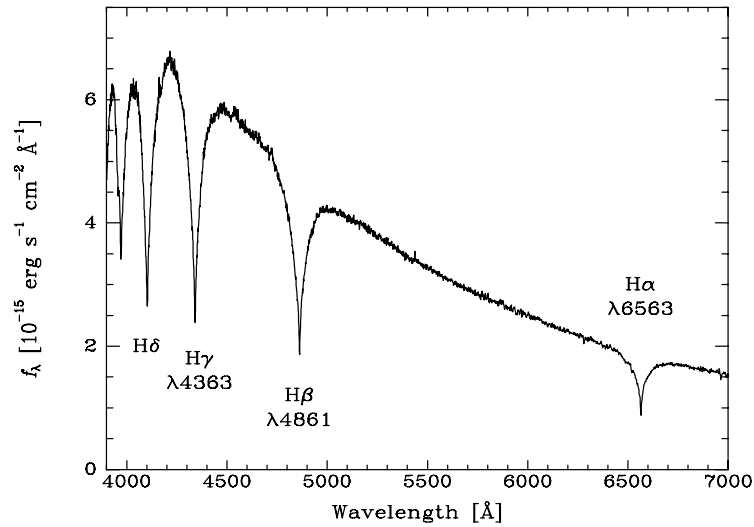
Figure 4.6 Optical-range spectrum of a typical DA-type white dwarf. Note the pressure-broadened hydrogen Balmer-line absorptions, reflecting the high surface gravity in the white-dwarf photosphere, superimposed on the blue thermal continuum. Data credit: Sloan Digital Sky Survey.
