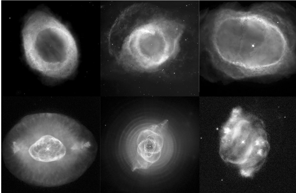
Figure 4.2 Several examples of planetary nebulae, newly exposed compact stellar cores that irradiate the shells of gas that were previously shed in the final stages of stellar evolution. The shells have diameters of \approx 0.2\text{--}1 pc. Photo credits: M. Meixner, T. A. Rector, B. Balick et al., H. Bond, R. Ciardullo, NASA, NOAO, ESA, and the Hubble Heritage Team.
