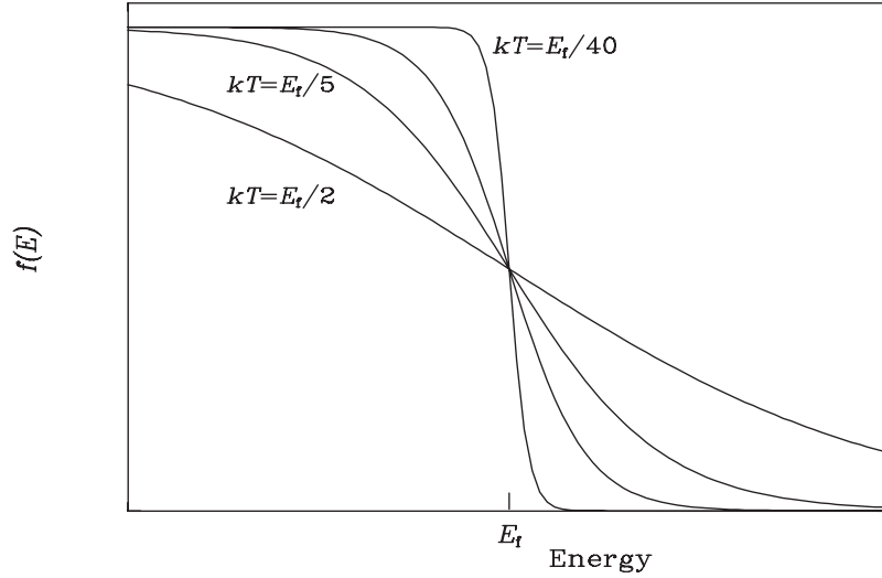
Figure 4.4 Approach to degeneracy of the Fermi–Dirac occupation number, f(E) , as kT \rightarrow 0 , shown for kT = E_F/2, E_F/5, E_F/10 , and E_F/40 . At kT \ll E_F , all particles occupy the lowest energy state possible without violating Pauli’s exclusion principle. The distribution then approaches a step function, with all energy states below E_F occupied, and all those above E_F empty.
