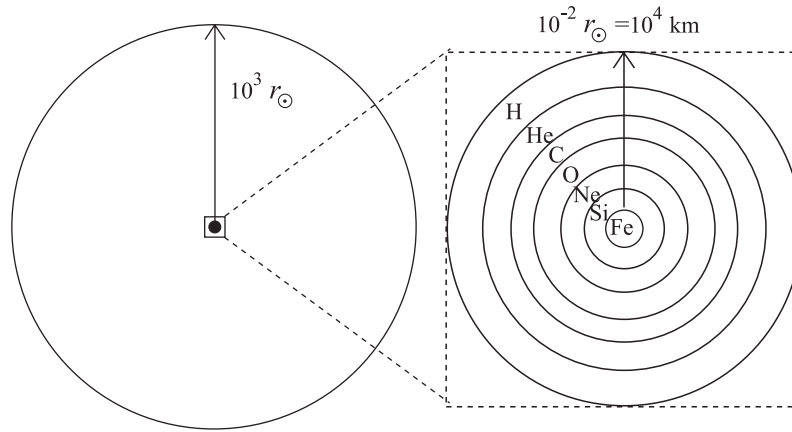
Figure 4.7 Simplified schematic view of the layered structure of a massive star and the distribution of the main elements that compose it, at the onset of core collapse and the ensuing supernova explosion.
