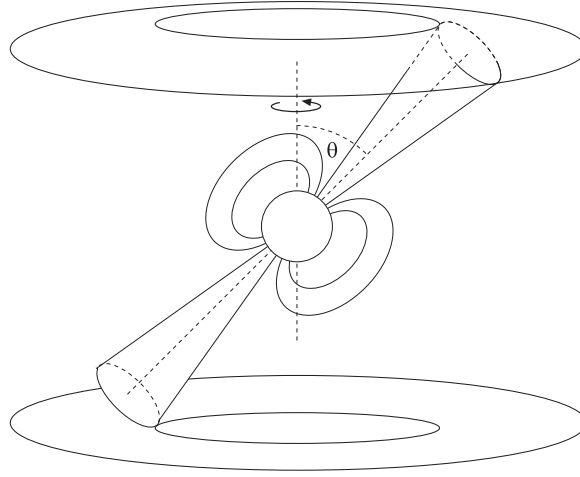
Figure 4.12 Schematic model of a pulsar. Biconical beams of radiation emerge along the magnetic axis of a neutron star. The magnetic axis is inclined by an angle \theta to the star's spin axis. Observers in a direction, as viewed from the star, that is within one of the two annular regions swept out by the beams as the star rotates will detect periodic pulses.
