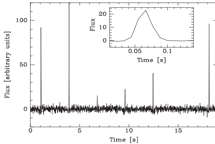
Figure 4.10 Flux at 430 MHz vs. time from PSR J0546+2441, a typical radio pulsar, over several periods. The pulse period is 2.84385038524 s (i.e., measured to 12 significant digits). Note the variable strength, and occasional disappearance of the pulses. The inset shows a zoom-in on the pulse profile, averaged over many periods. Data credit: D. Champion, see Mon. Not. Royal Astron. Soc. (2005), 363, 929.
