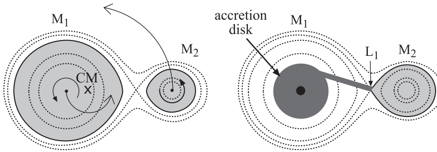
Figure 4.13 Equipotential surfaces (dotted curves) in the corotating reference frame of a binary system with mass ratio M_1/M_2 = 5 . Left: In this example, both stars are inside their respective Roche lobes, but are tidally distorted. Loss of energy to tidal friction will cease only when the orbits about the center of mass become circularized, and aligned and synchronized with the rotations, so that there is no motion in the corotating frame. Right: Here, the secondary star, on the right, fills its Roche lobe. Matter flows through the L_1 point and falls onto the primary star, which is now a compact object. Viewed from an inertial frame, the falling material possesses angular momentum, and hence an accretion disk is formed around the compact primary star.
